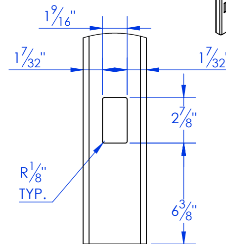
DETAIL A SCALE 1 : 6
